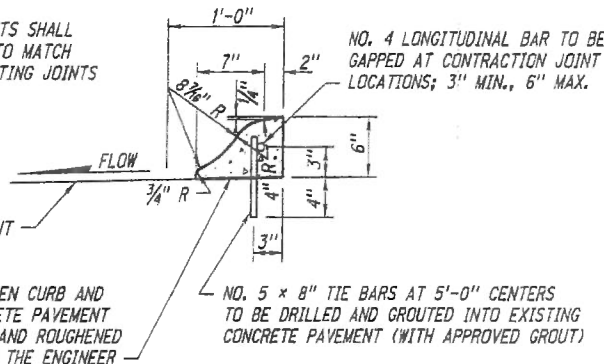
CONCRETE CURB, * TYPE II
