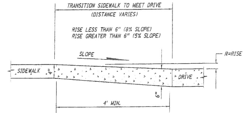
SECTION G-G
