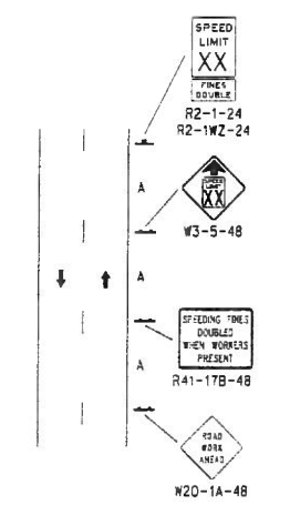
TYPICAL ADVANCED SIGNING
